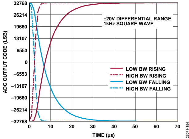
Figure 63. Step Response, ±20 V Differential Range
