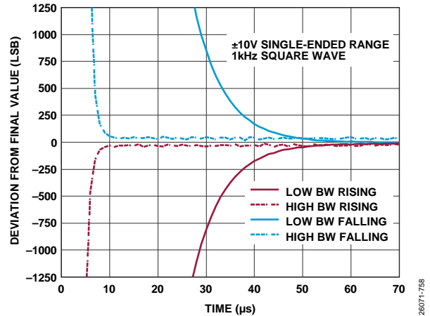
Figure 67. Step Response, ±10 V Single-Ended Range, Fine Settling
