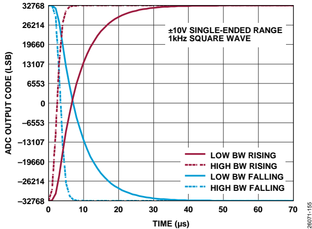
Figure 64 Step Response, ±10 V Single-Ended Range
