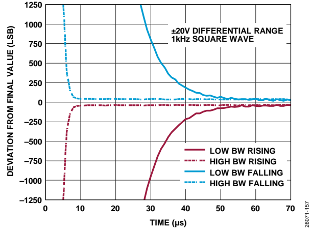
Figure 66. Step Response, ±20 V Differential Range, Fine Settling
