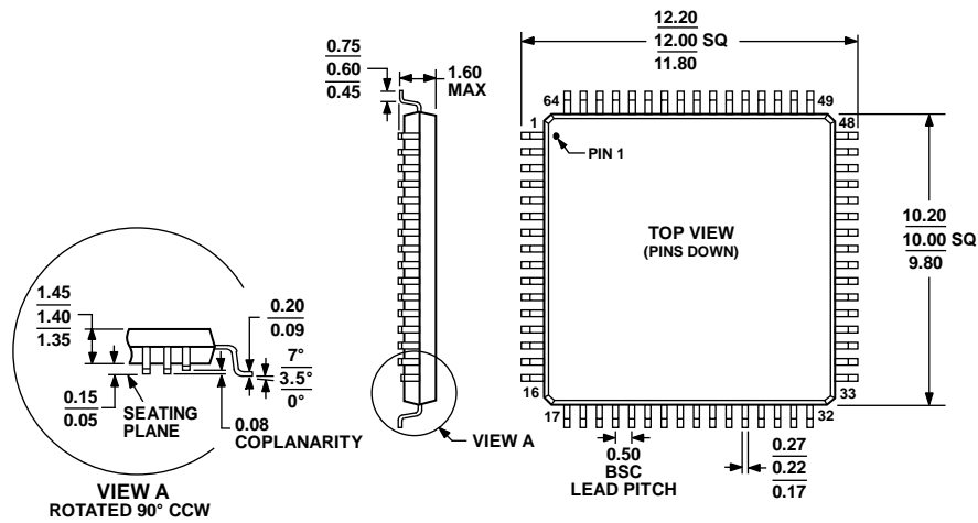
Figure 125. 64-Lead Low Profile Quad Flat Package [LQFP] (ST-64-2)
